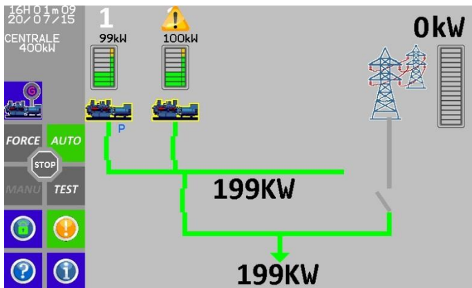
2 gensets power station synoptic
